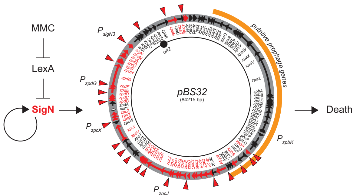
FIG 7 Model of pBS32-mediated cell death. MMC-mediated DNA damage causes LexA autoproteolysis and derepression of sigN expression. SigN is a sigma factor that directs RNA polymerase to increase its own expression (creating positive feedback) and the expression of a regulon of genes on pBS32. Activation of genes within the SigN regulon results in cell death. pBS32 is represented as a circle. Arrows within the circle indicate reading frames. The location of SigN-dependent promoters is indicated by red arrowheads. Reading frames and gene names that are expressed by SigN are indicated in red. T bars indicate inhibition, and arrows indicate activation. In black are the locations of specific promoters mentioned in the text.
