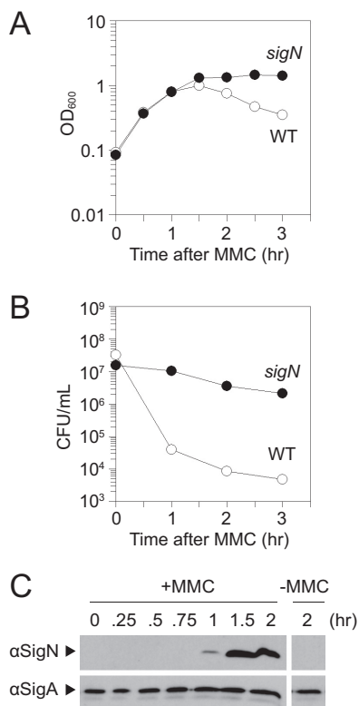
FIG 1 SigN is required for loss of cell viability after MMC treatment. (A) Optical density ( OD_{600} ) growth curve of wild type (open circles, DK607) and sigN mutant (closed circles, DK3287). The x axis is the time of spectrophotometry after MMC addition. (B) CFU growth curve of wild type (open circles, DK607) and sigN mutant (closed circles, DK3287). The x axis is the time of dilution plating after MMC addition. (C) Western blot analysis of wild-type DK607 cell lysates harvested at the indicated time after MMC addition and probed with either anti-SigN antibody or anti-SigA antibody. On the right is a single panel of the same strain for comparison 2 h after mock MMC addition.
